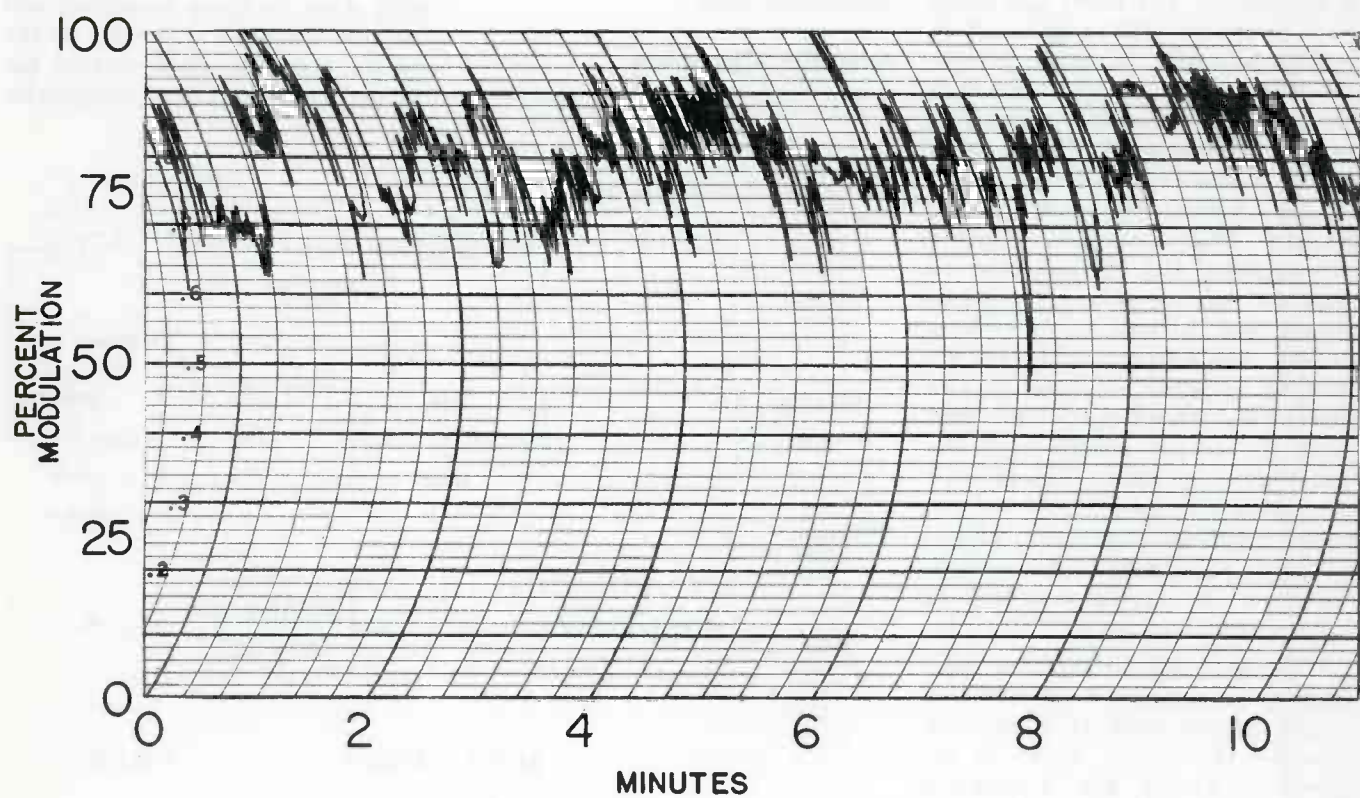
Figure 5 Recording of limiter output without AGC amplifier.
