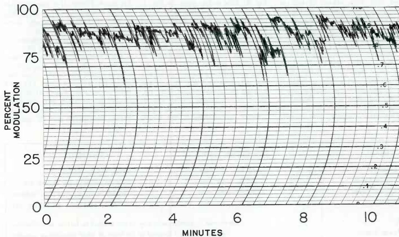
Figure 7 Limiter plus AGC amplifier. Note smoothness of operation compared with other curves.
